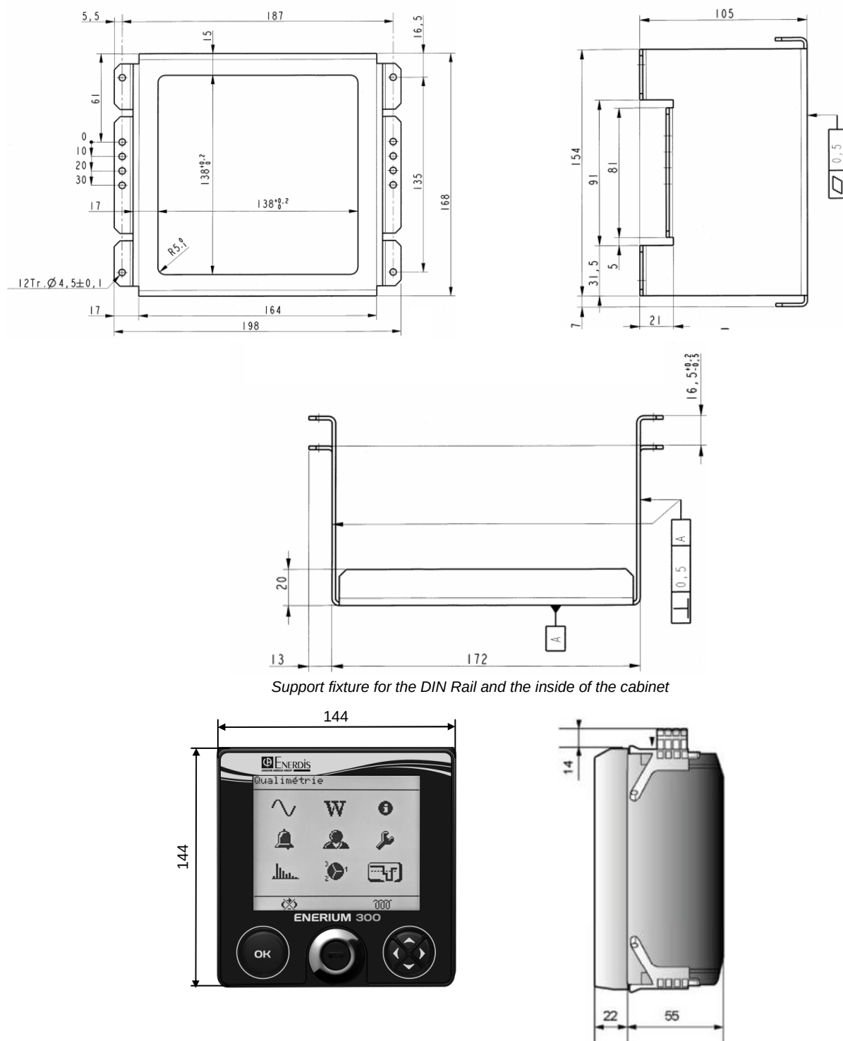
Overall dimensions in millimetres
