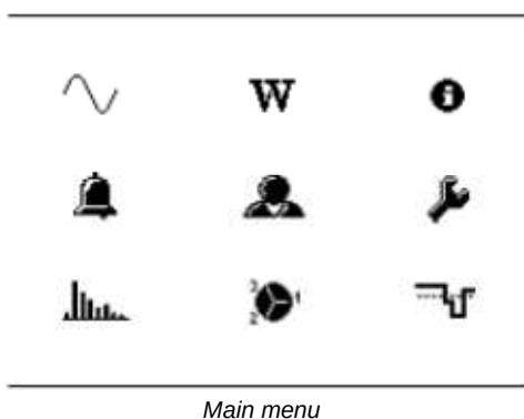
Main menu
