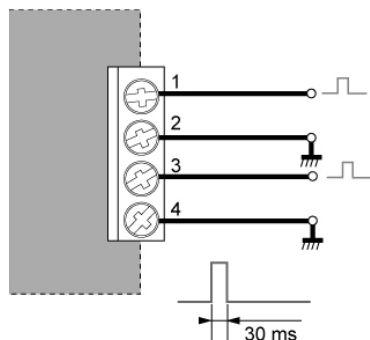
Example of digital output connections in impulse mode.
